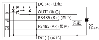
◎ PNP + RS485
